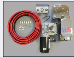
Electric Motor Conversion with Easy Switch Kit
