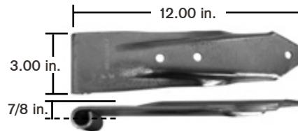
Swing Door Hinge, 3-Hole Material: Steel
