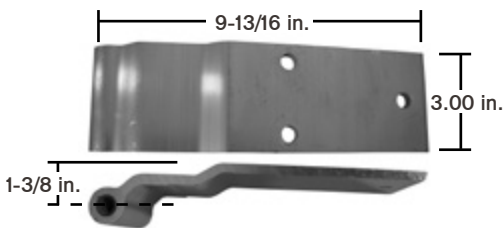
Swing Door Hinge, 3-Hole, Includes Bushing Material: Aluminum
