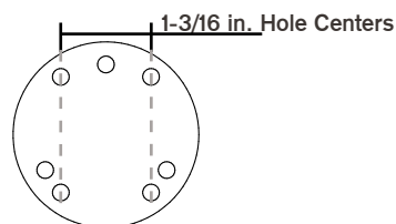
Ram Mount Washer, Diameter: 2-7/16in. Material: Steel, 10ga.
