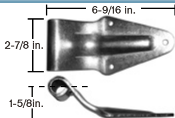
Swing Door Hinge, 3-Hole Material: Steel
