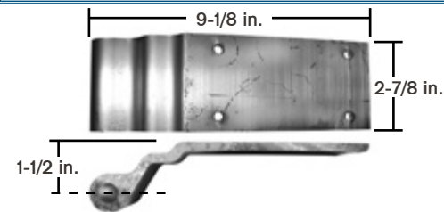
Swing Door Hinge, 4-Hole Material: Aluminum
