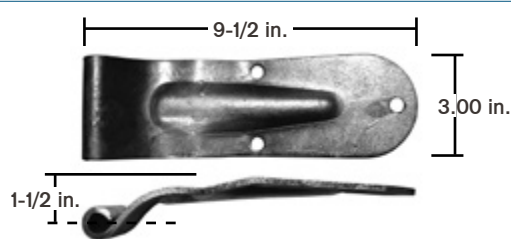
Swing Door Hinge, 3-Hole Material: Steel
