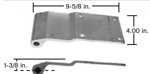
Swing Door Hinge, 4-Hole Material: Aluminum
