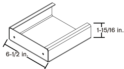
PeopleNet Keyboard Mount Material: Steel, Black Powder Coat
