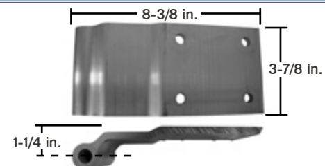
Swing Door Hinge, 4-Hole Material: Aluminum
