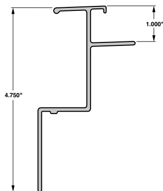
Top Rail GVFD
