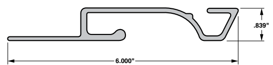
Side Door Frame L/S GVFD Current
