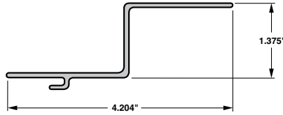
Connector Post GVSD
