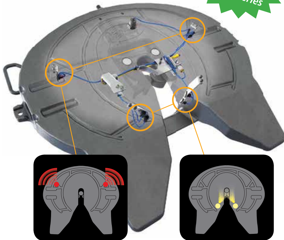
FAILED MODE Red Flashing Warning Lights
