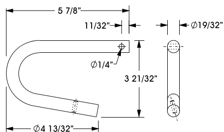
MODEL 1269-R HANDLE
